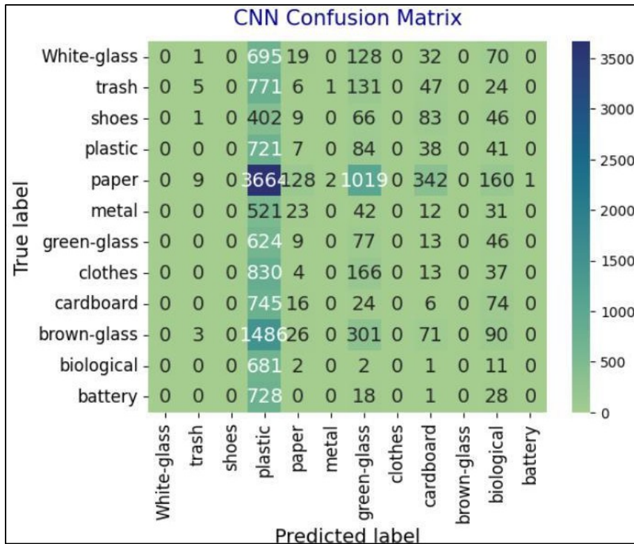
Graph 3 : CNN matrix
