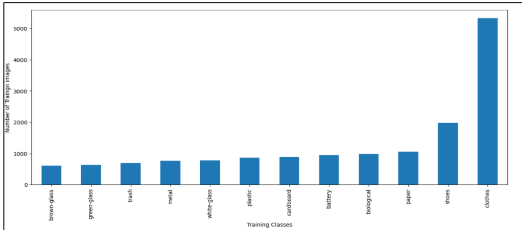
Graph 1 : Dataset
